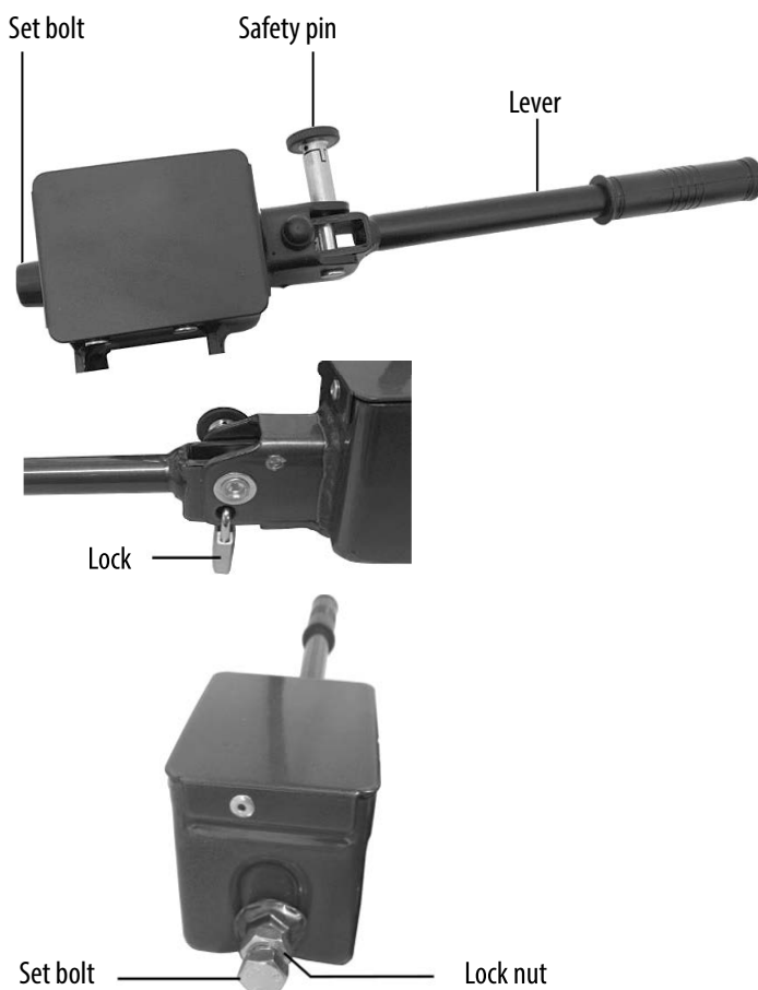
Figure 7: Quick closure
