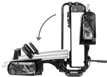
Figure 8: Step 1
