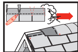
On ridges cut the tabs as shown
