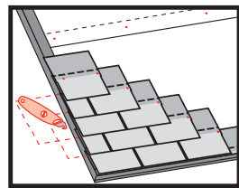
Cut the tabs as shown for correct application
