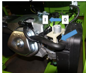
Throttle valve to position 0 for starting. To Pos. I during operation.
