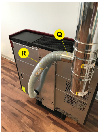
Fig. 11 - Anschlüsse
