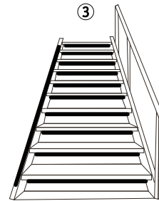
A step strips + B side strip MAX. 18 steps MAX. 10m
